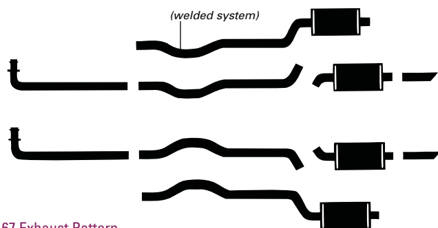
63-67 Exhaust Pattern
