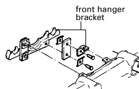
front hanger bracket
