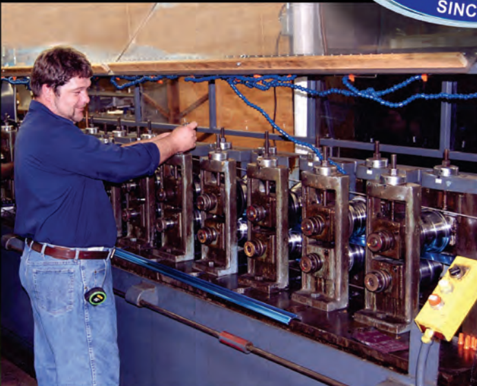
This 20 station roll forming mill is one of three used at Dennis Carpenters to make classic Ford car and truck parts
