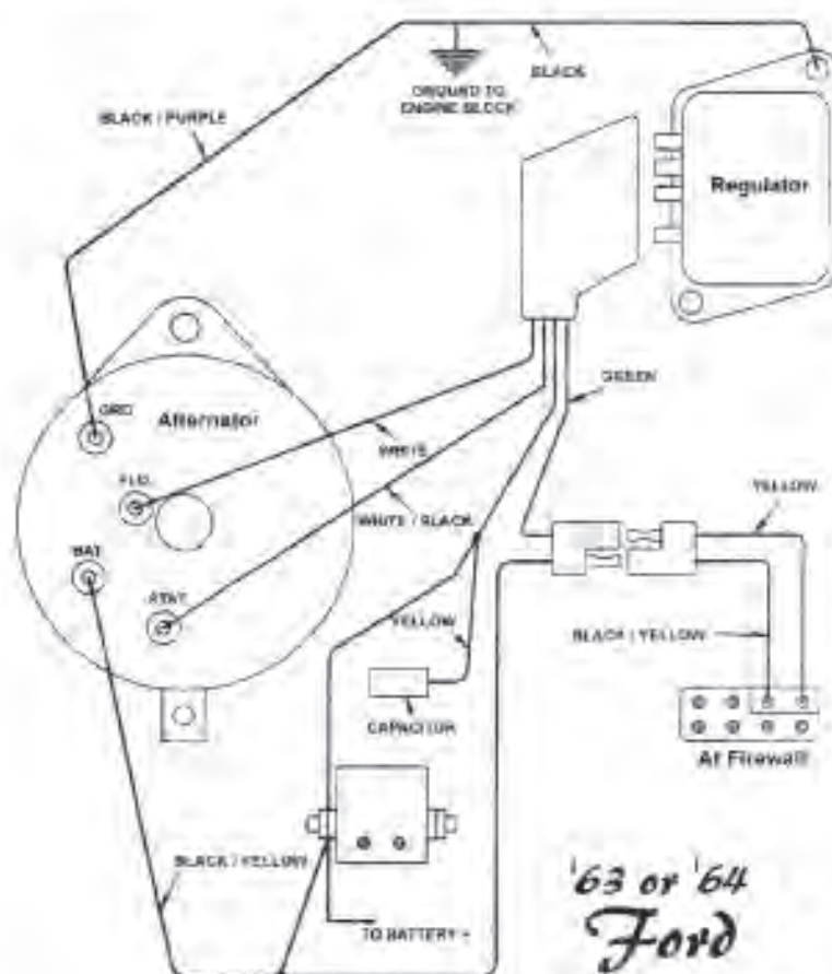
Conversion from Generator Charging System to Alternator Charging System
