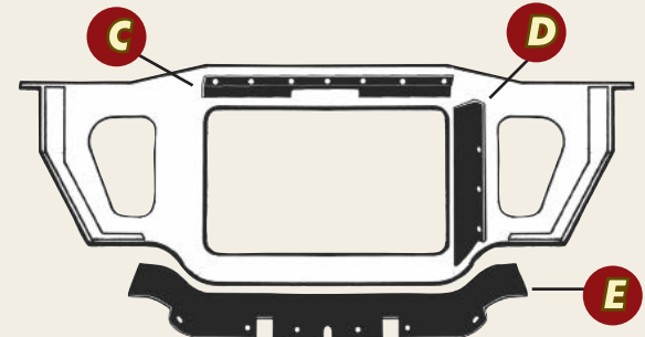
back of radiator support (engine side)
