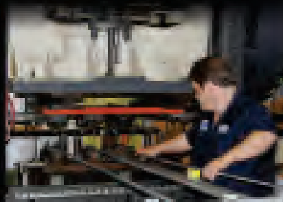
This press is fitted with a 3-stage progressive stamping die that makes 1977-79 F-100 hood-trunk moldings.
