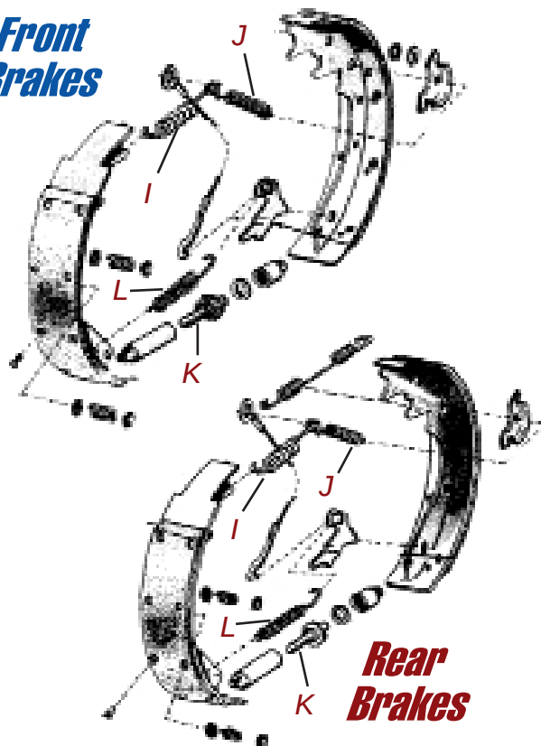
Front & Rear Drum Brakes - (Self Adjusting)
