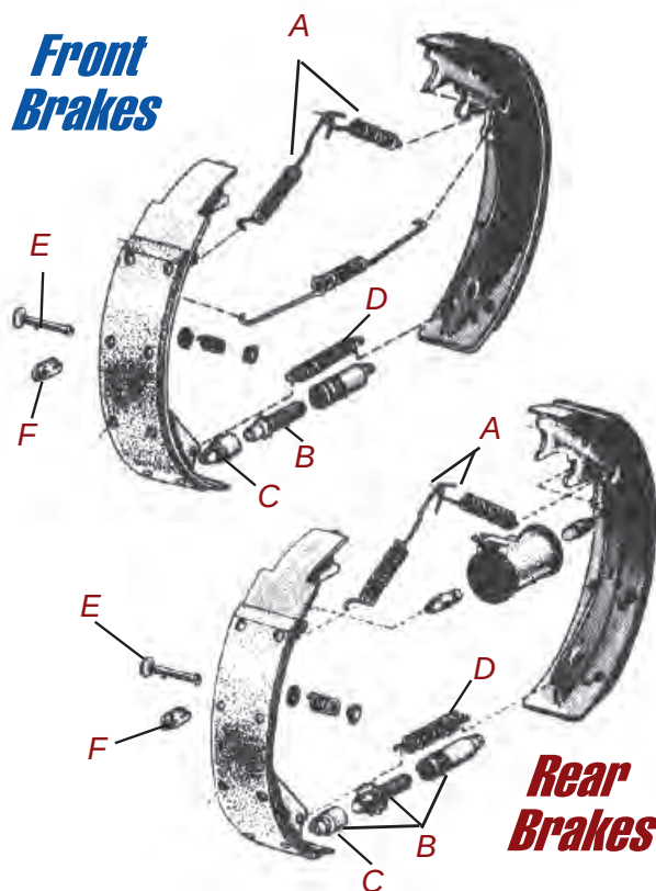
Front & Rear Drum Brakes - (Manual Adjusting)
