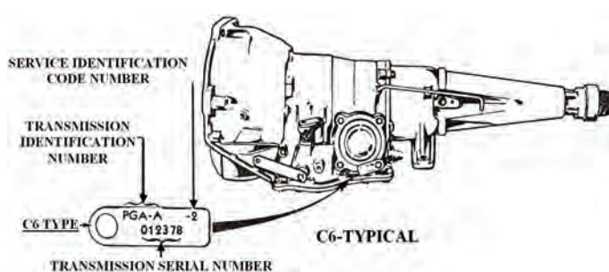
C6-TYPICAL
