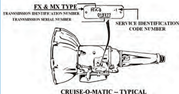
CRUISE-O-MATIC - TYPICAL
